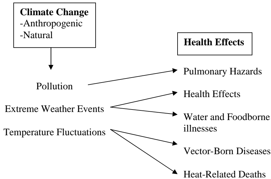
Figure 5.1 Potential relationships between certain naturally induced and anthropogenic climate changes and the health effects they generate.
