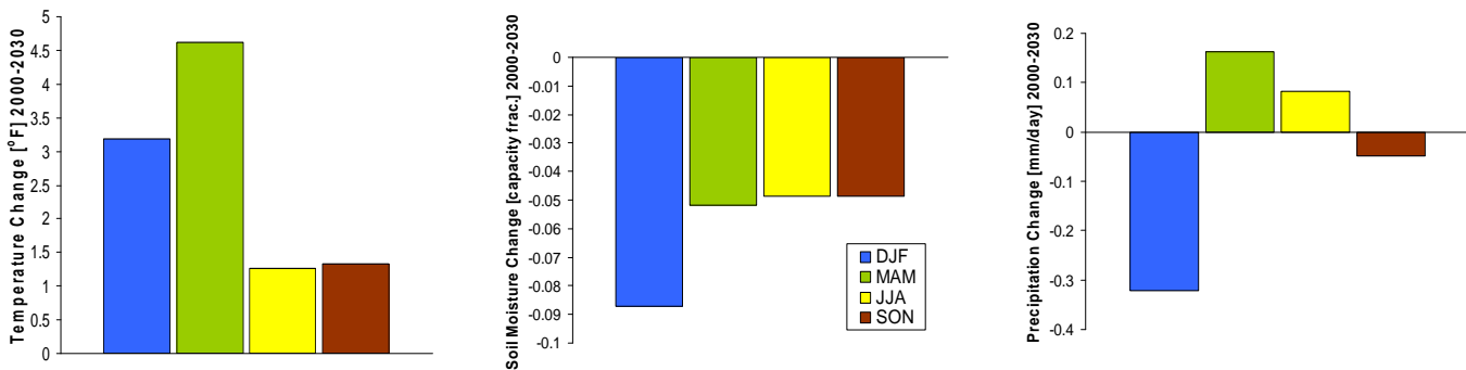
Figure 2.5. Climate change 2000-2030 for grid representing area around Cincinnati. Average of three runs CGCM2 GHG+A IS92a scenario, December – February (DJF), March – May (MAM), June - August (JJA), and September – October (SON). Soil moisture was predicted as capacity fraction, precipitation was predicted as mm/day, and the temperature as screen temperature (2m) in °C, which was converted to F.
